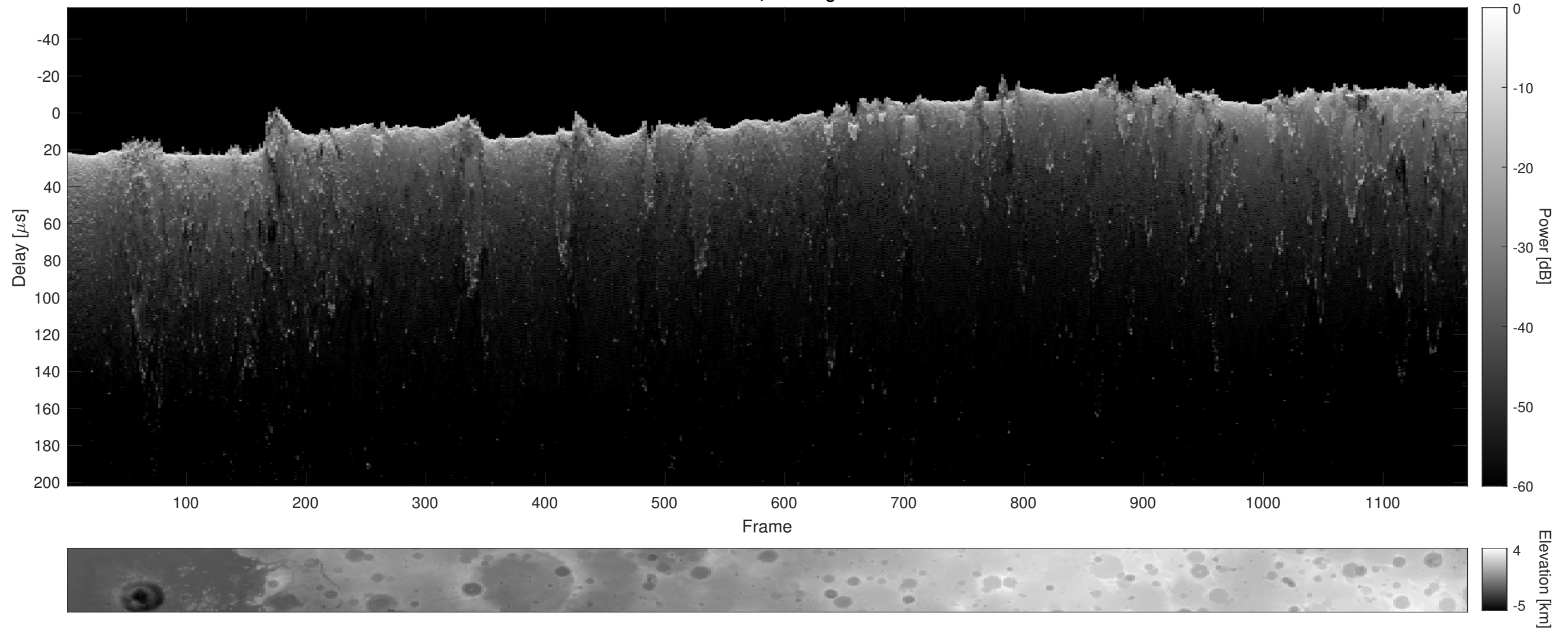
Orbit 21865, Cluttergram
