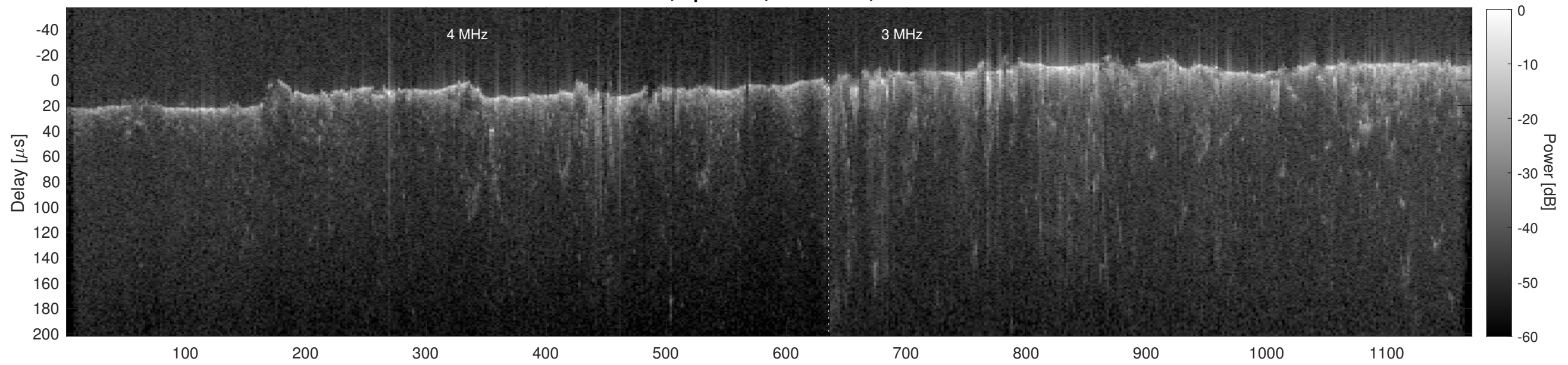
Orbit 21865, Cluttergram
