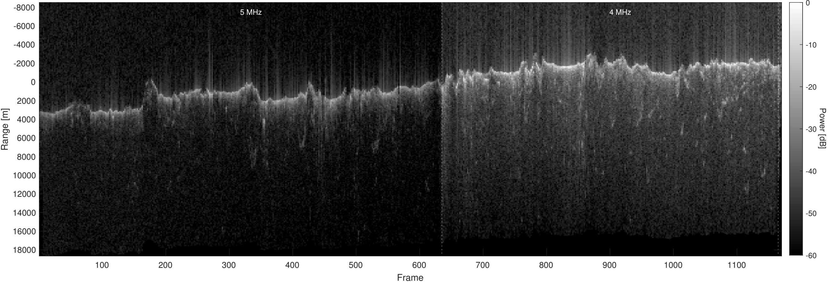
Orbit 21865, Optimized, No Window, Depth-Corrected, Channel 2
