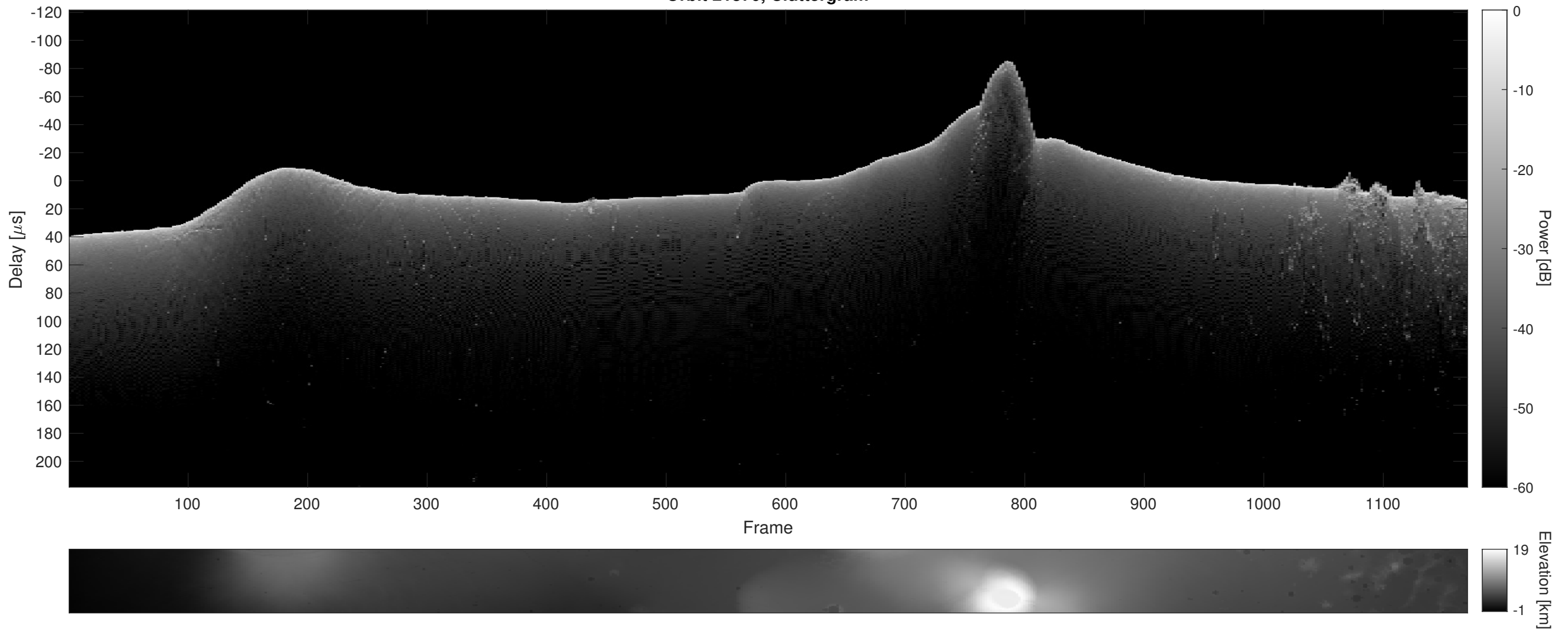
Orbit 21870, Cluttergram
