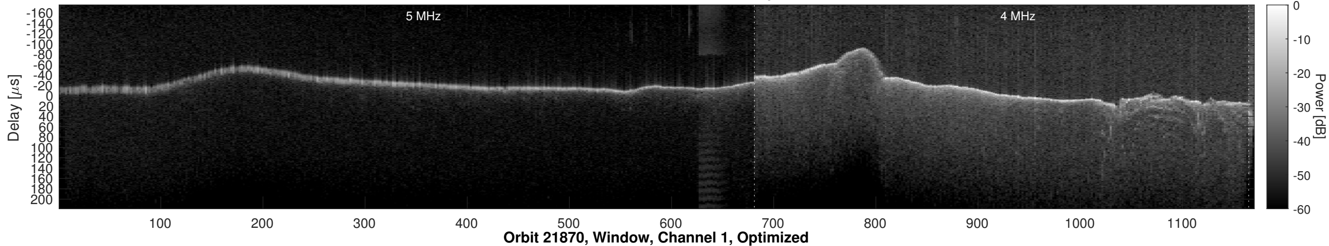
Orbit 21870, Window, Channel 1, Chapman
