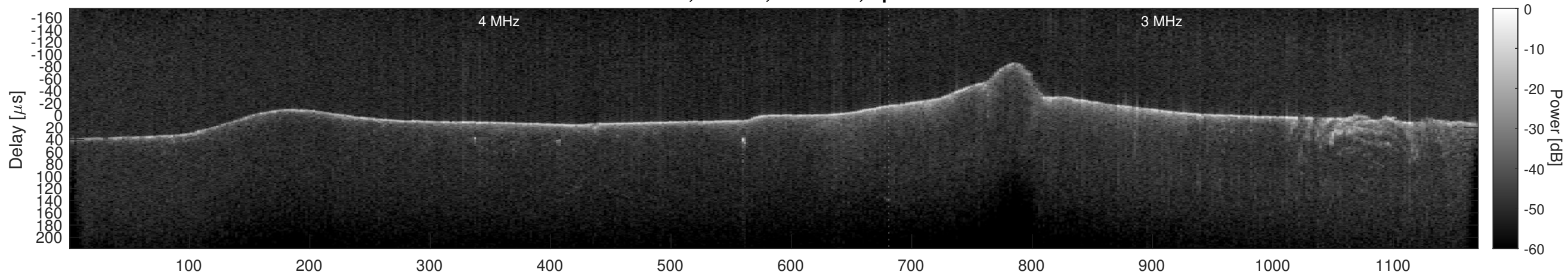
Orbit 21870, Cluttergram
