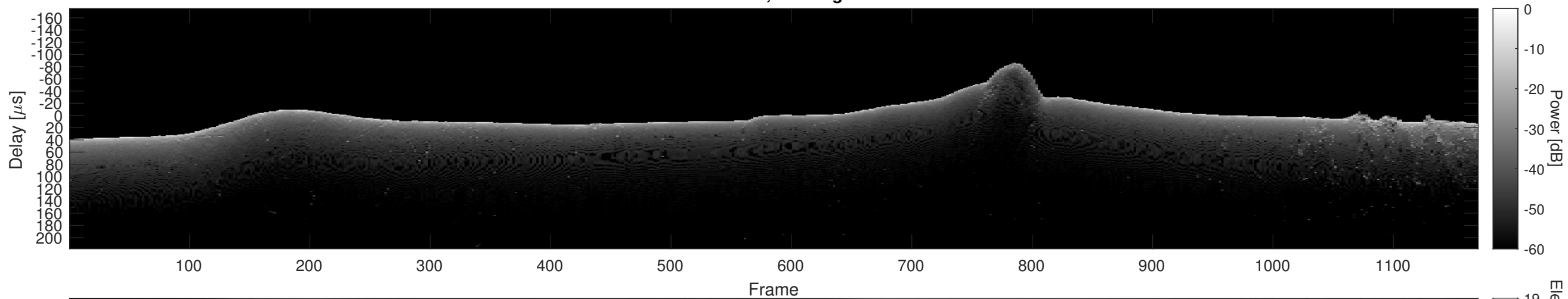
Orbit 21870, Cluttergram
