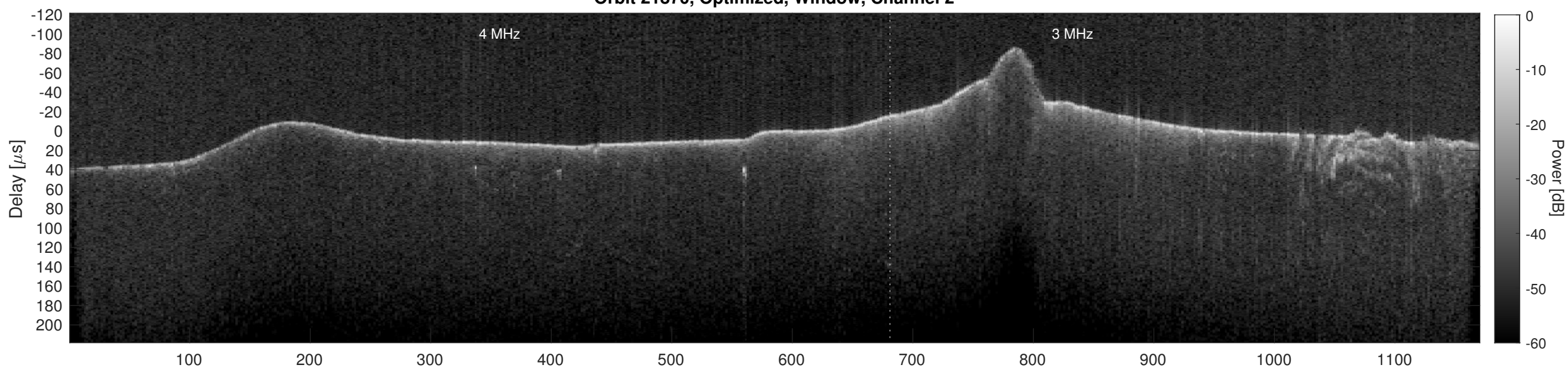
Orbit 21870, Cluttergram
