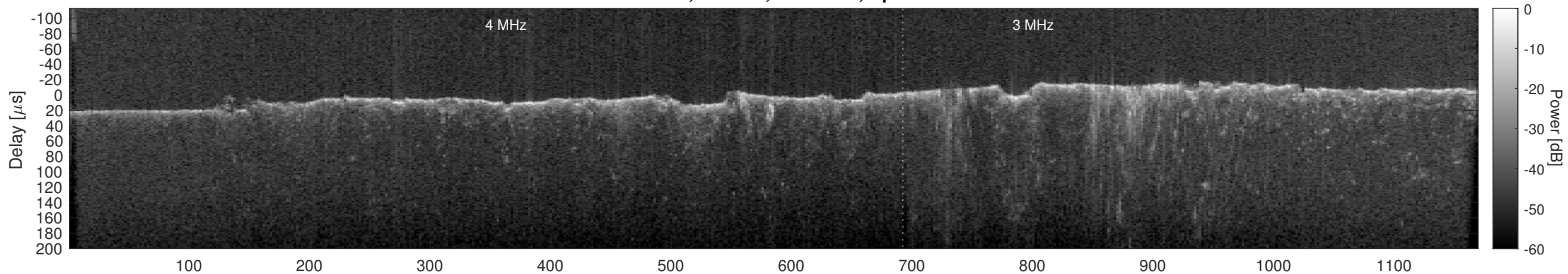
Orbit 21872, Cluttergram
