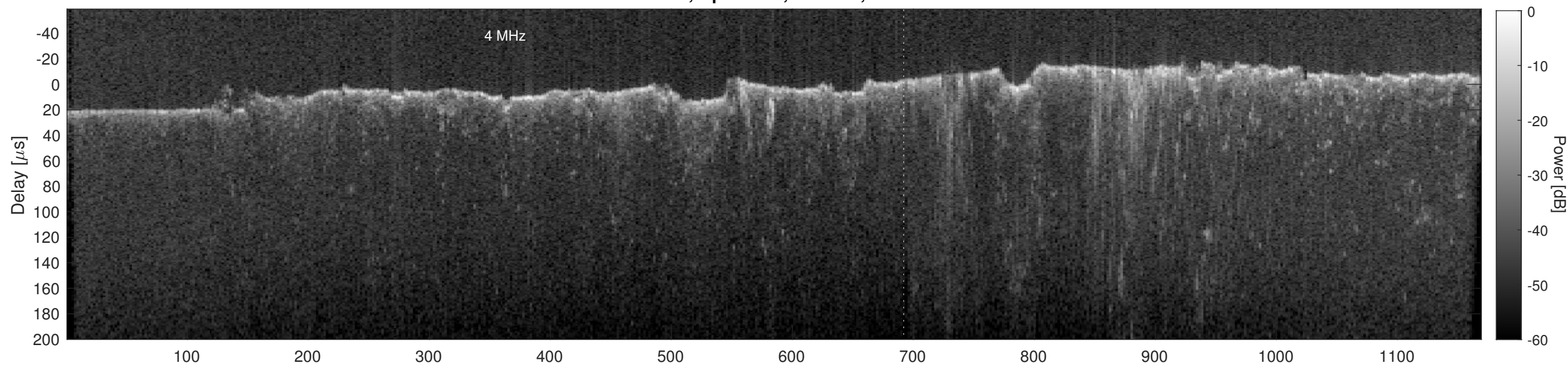
Orbit 21872, Cluttergram
