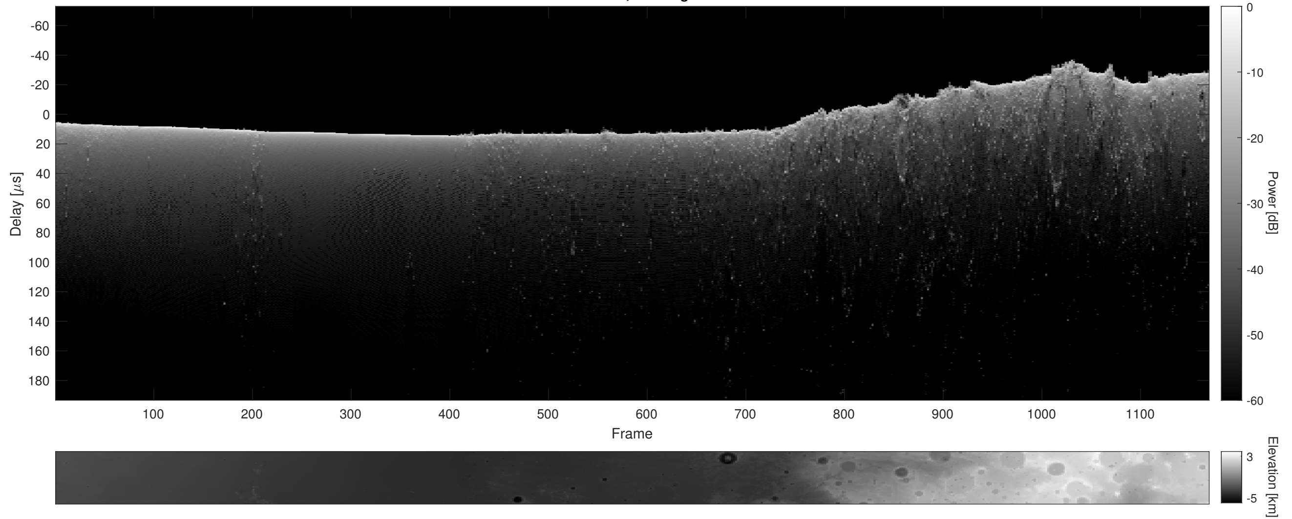
Orbit 21874, Cluttergram
