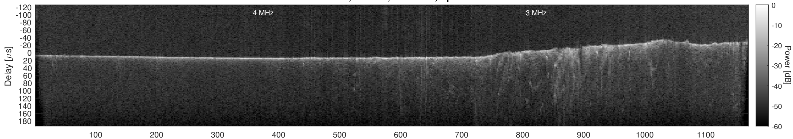
Orbit 21874, Cluttergram
