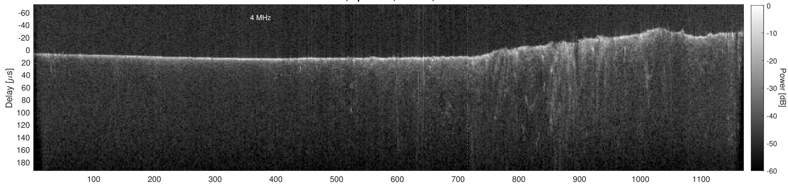
Orbit 21874, Cluttergram
