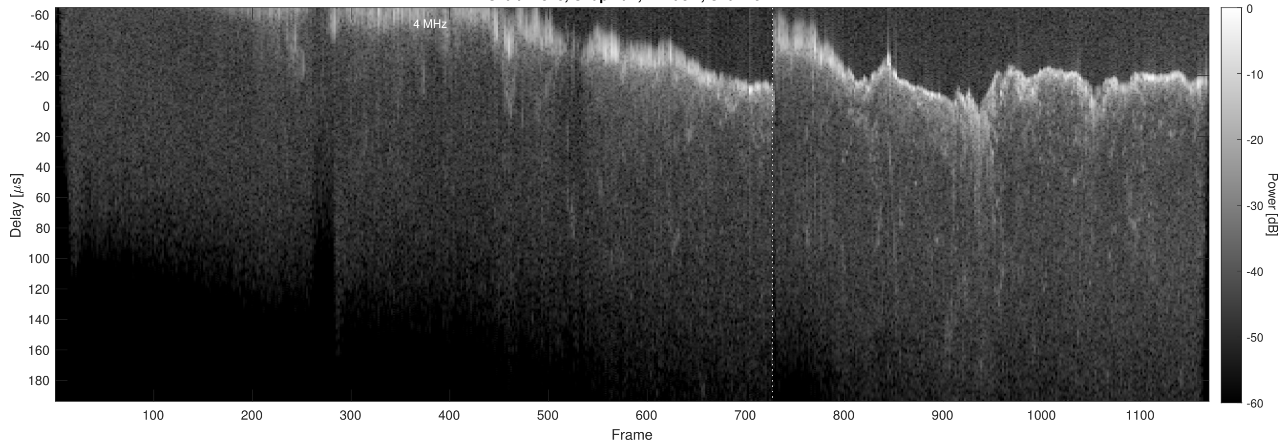
Orbit 21876, Chapman, Window, Channel 2
