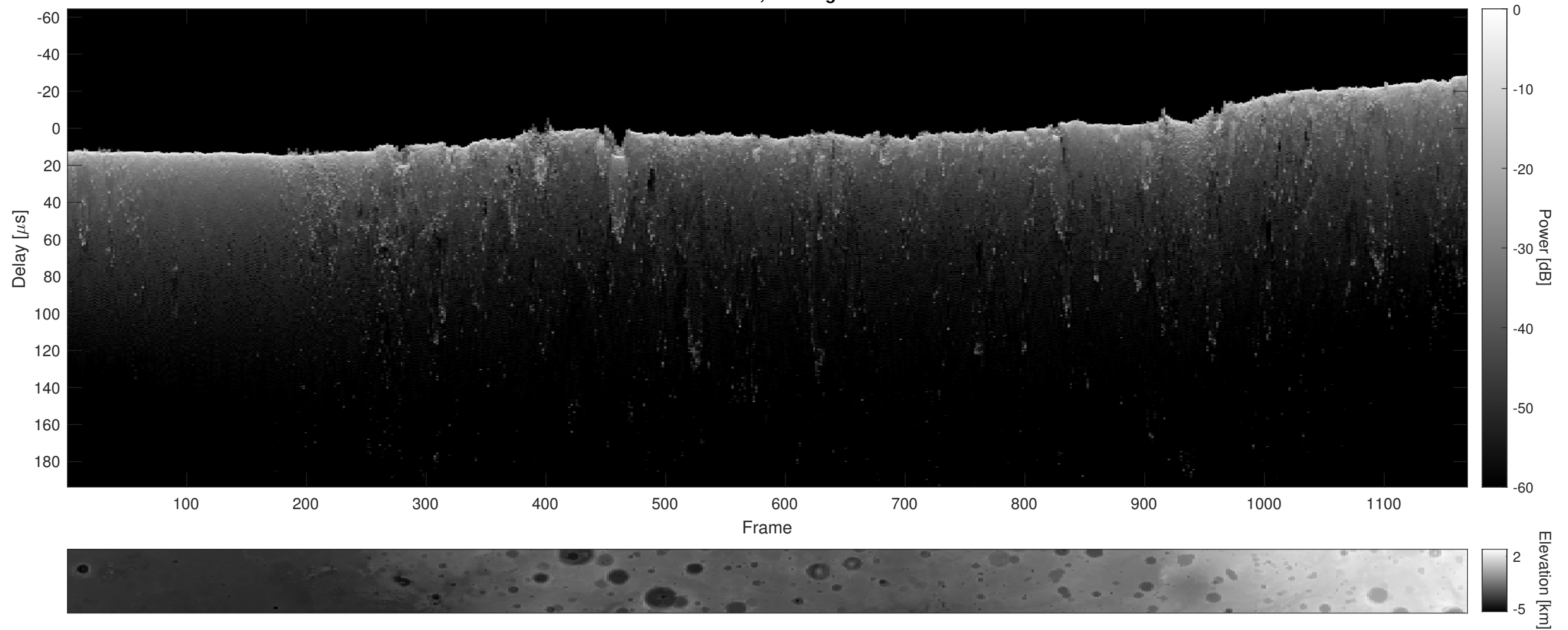
Orbit 21876, Cluttergram
