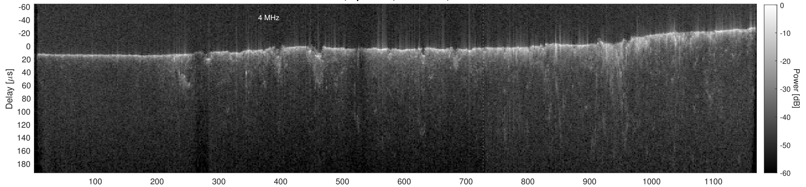
Orbit 21876, Cluttergram
