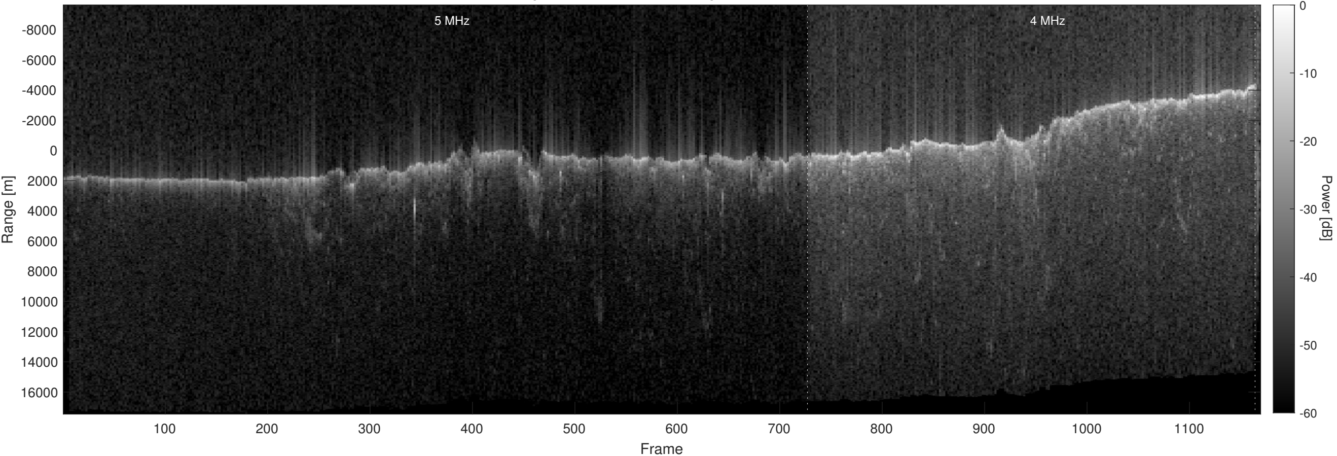
Orbit 21876, Optimized, No Window, Depth-Corrected, Channel 2
