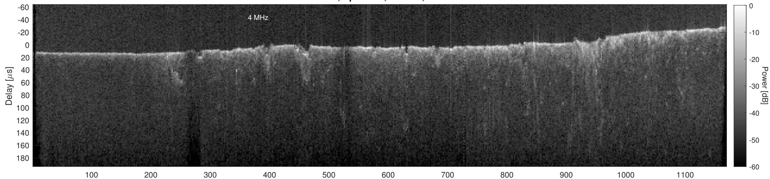
Orbit 21876, Cluttergram
