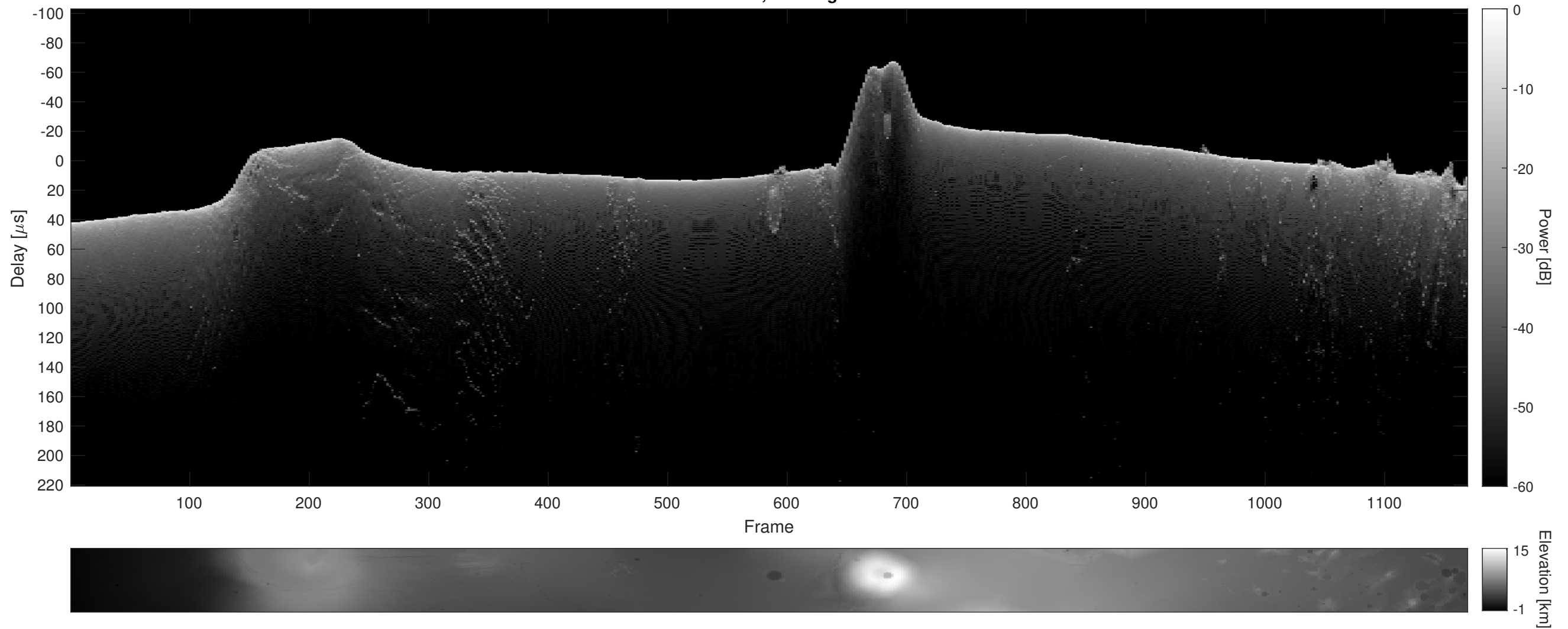
Orbit 21877, Cluttergram
