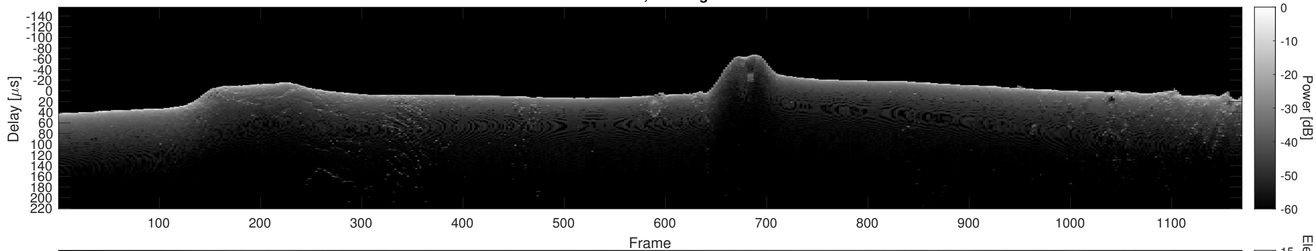
Orbit 21877, Cluttergram
