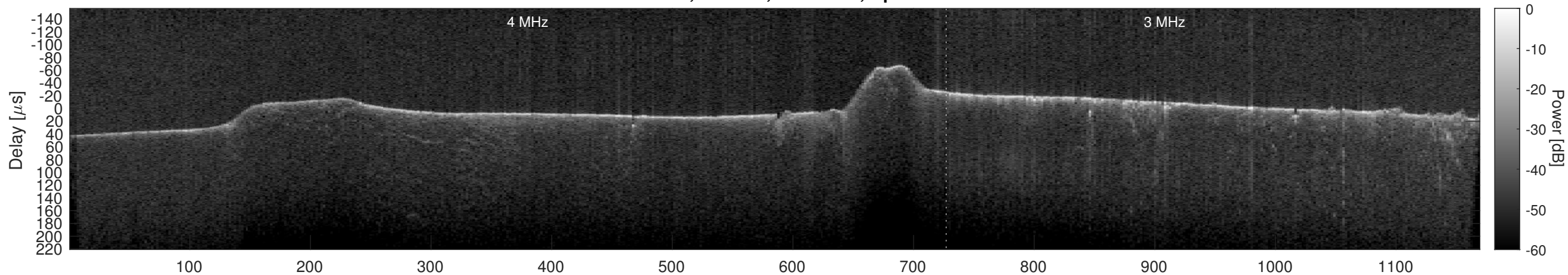
Orbit 21877, Cluttergram
