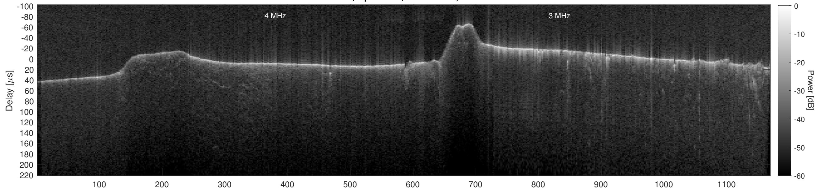
Orbit 21877, Cluttergram
