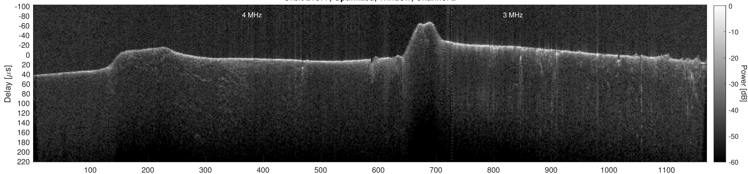
Orbit 21877, Cluttergram
