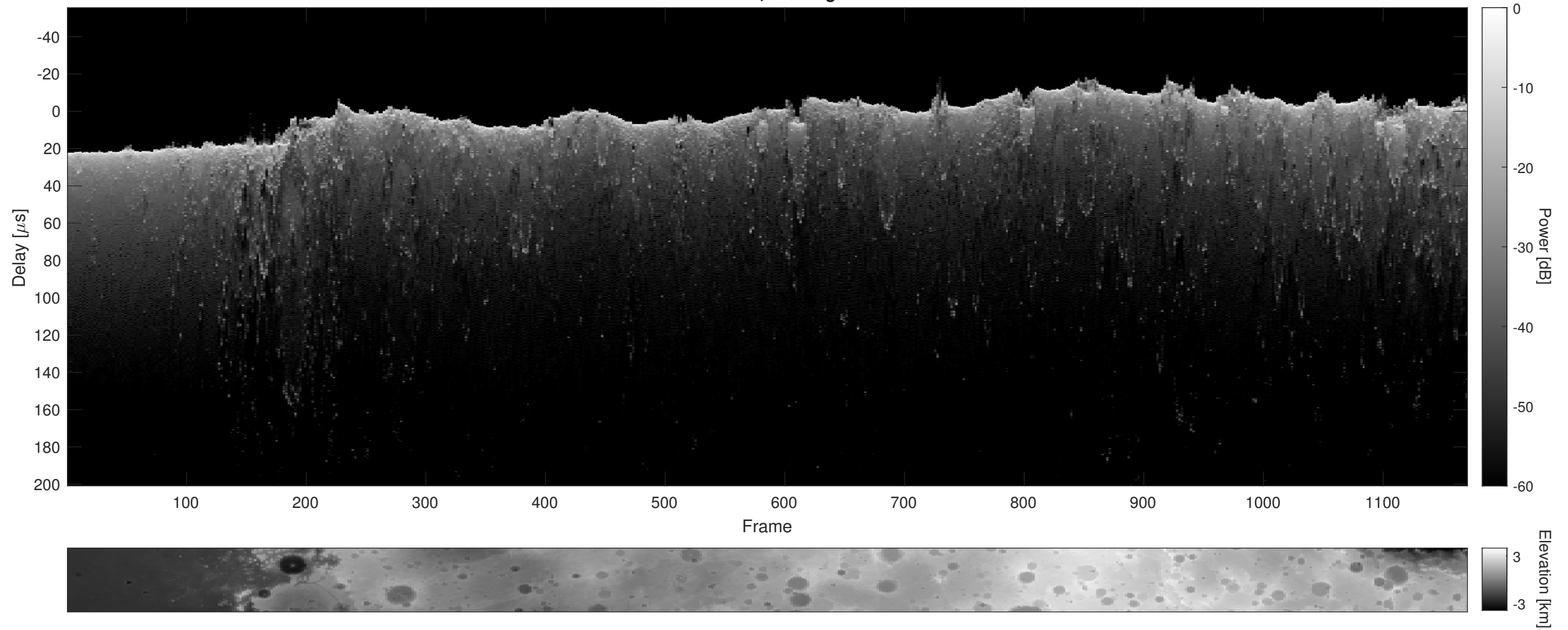
Orbit 21879, Cluttergram
