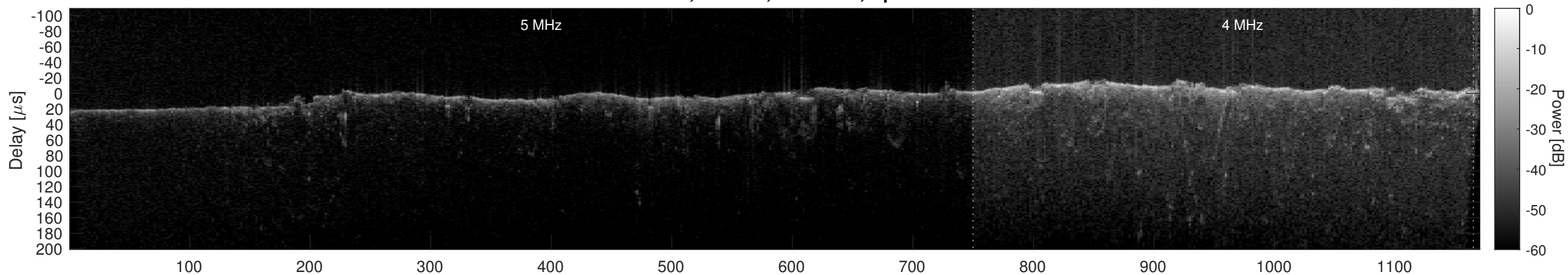
Orbit 21879, Cluttergram
