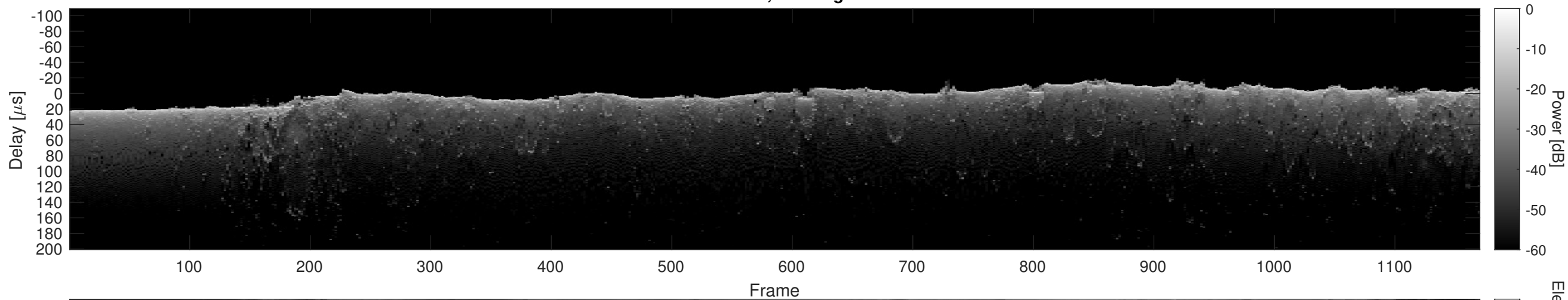
Orbit 21879, Cluttergram
