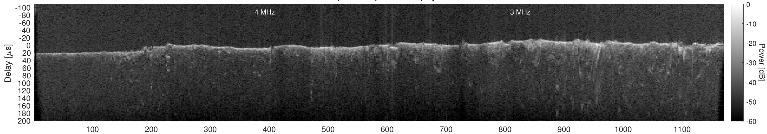
Orbit 21879, Cluttergram
