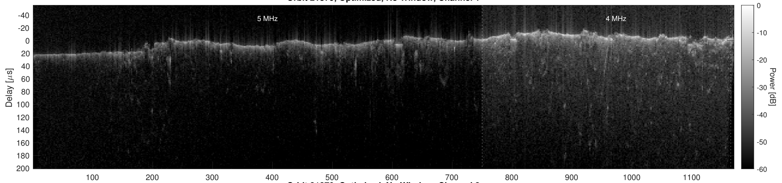
Orbit 21879, Optimized, No Window, Channel 2
