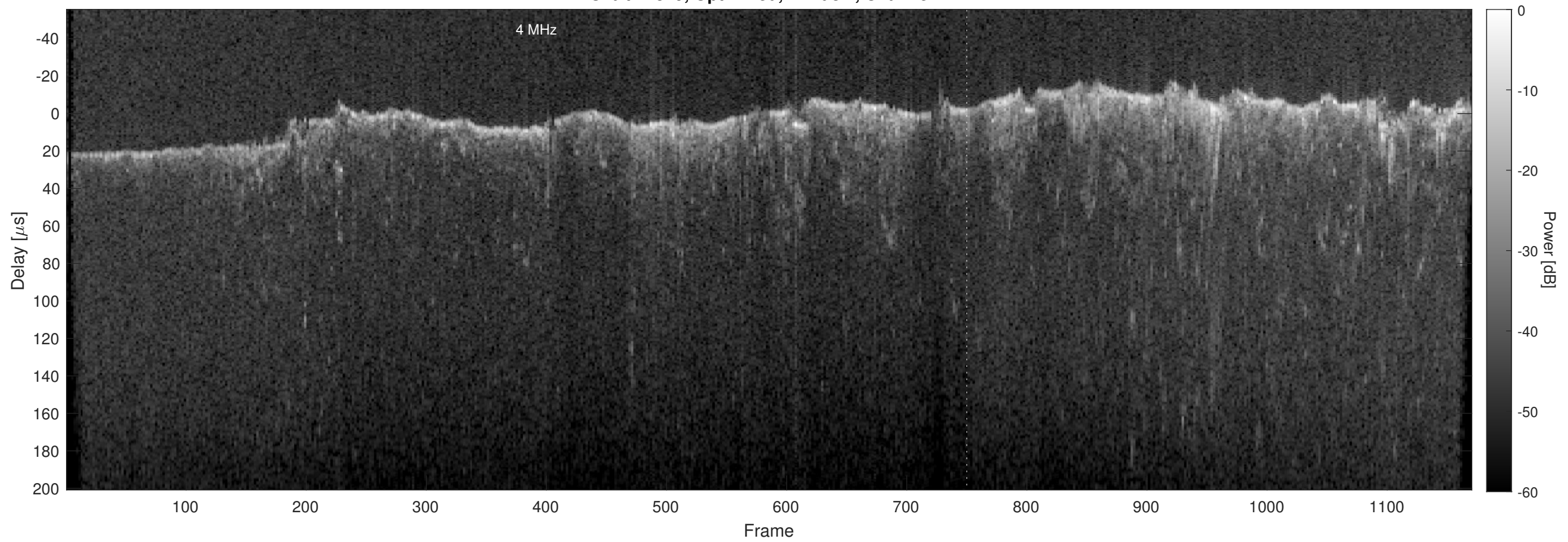
Orbit 21879, Optimized, Window, Channel 2
