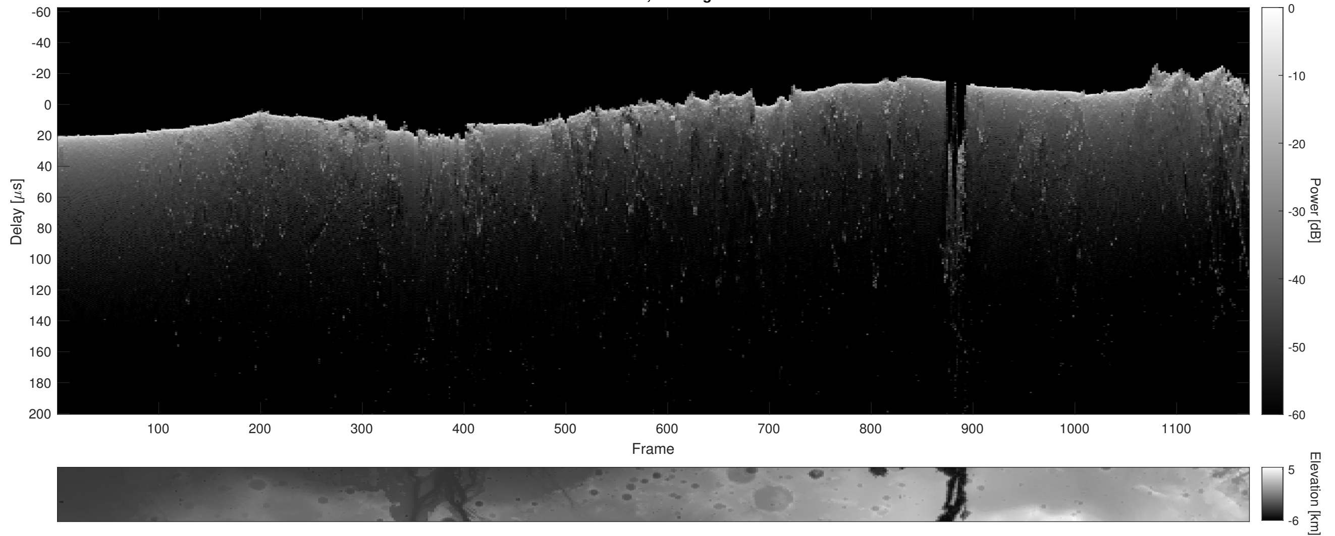
Orbit 21887, Cluttergram
