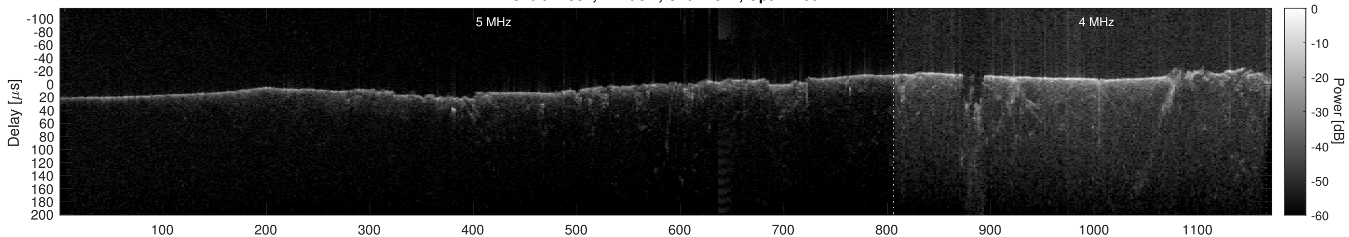
Orbit 21887, Cluttergram
