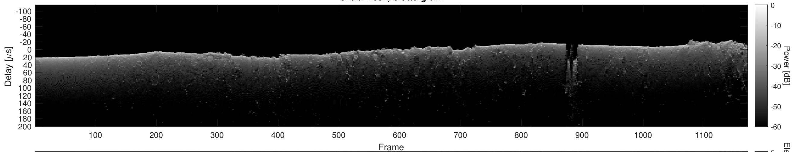
Orbit 21887, Cluttergram
