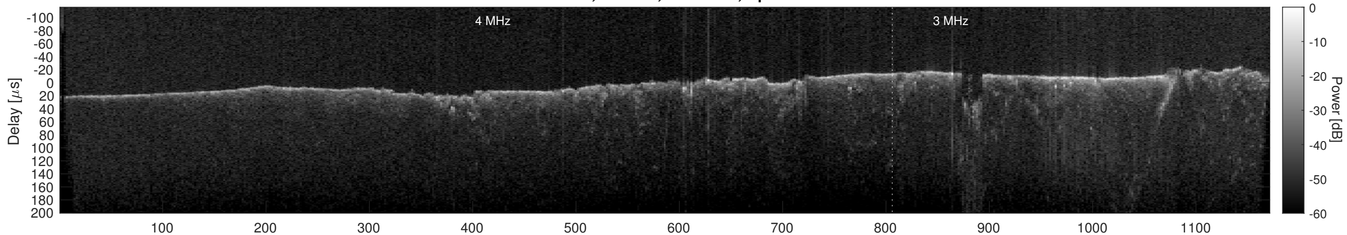
Orbit 21887, Cluttergram
