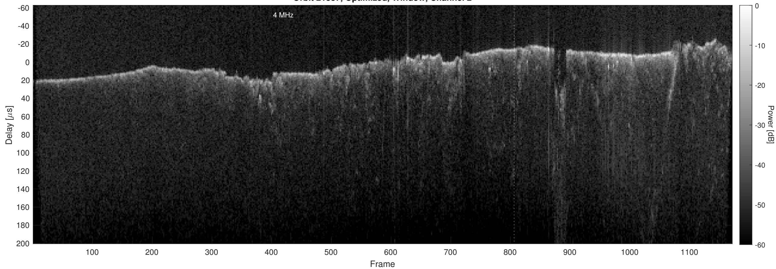
Orbit 21887, Optimized, Window, Channel 2
