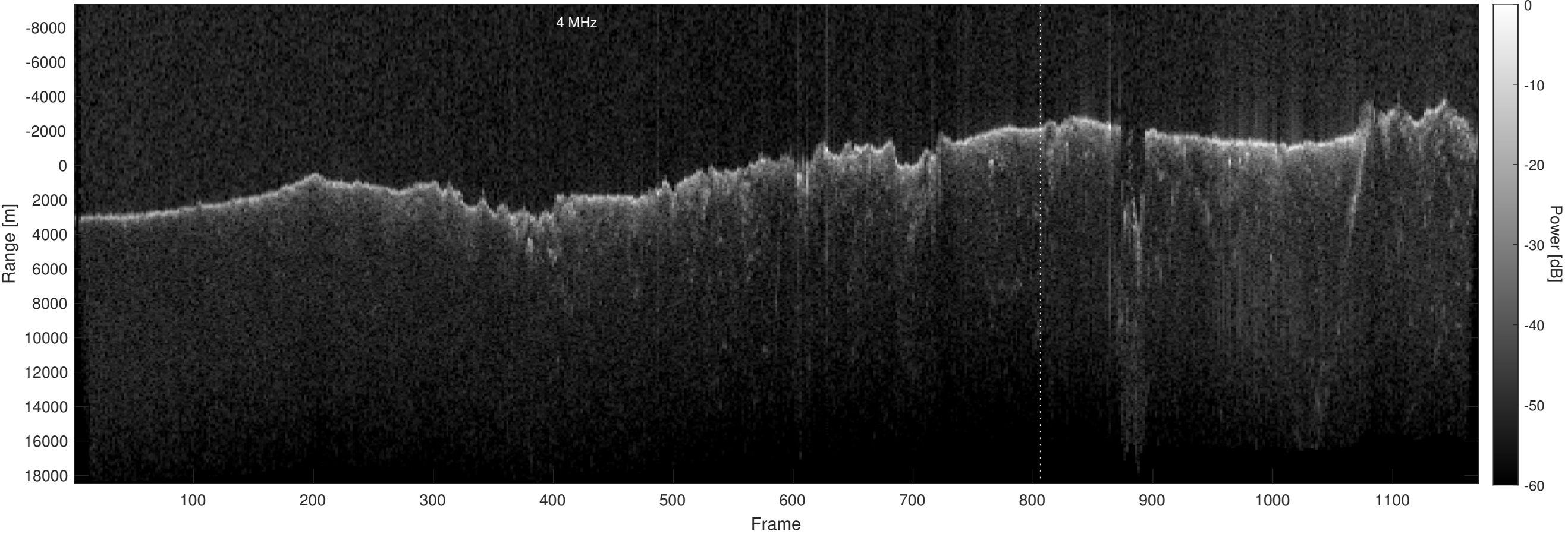
Orbit 21887, Optimized, Window, Depth-Corrected, Channel 2
