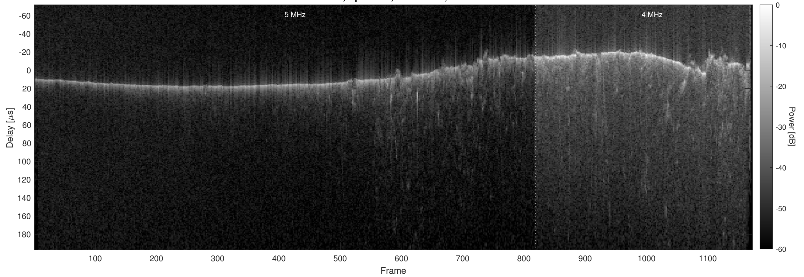
Orbit 21889, Optimized, No Window, Channel 2
