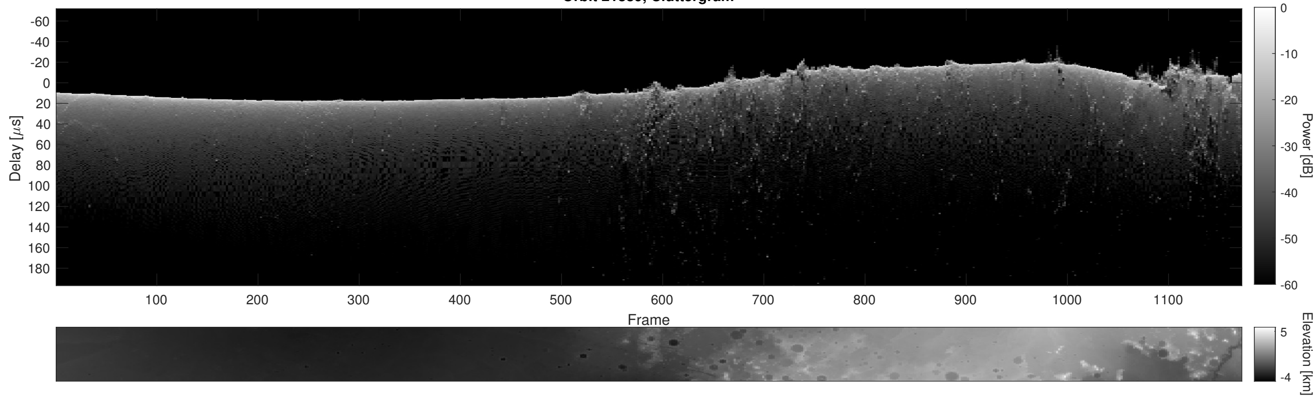
Orbit 21889, Cluttergram
