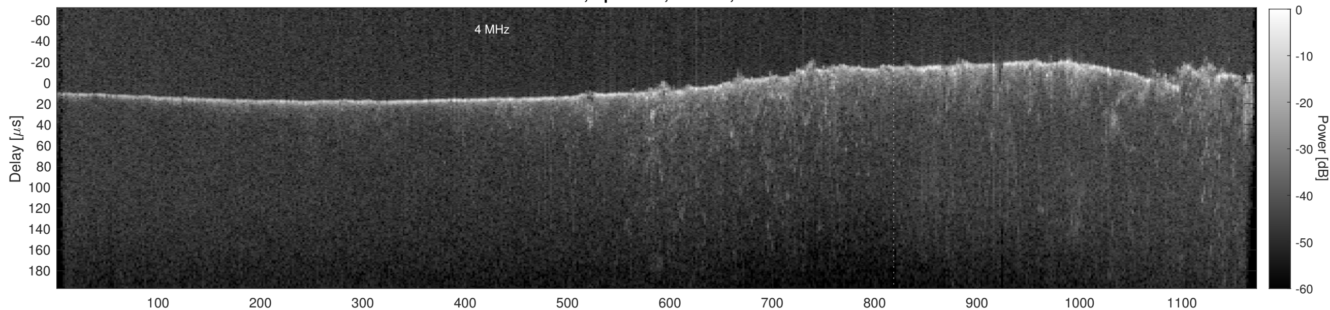
Orbit 21889, Cluttergram
