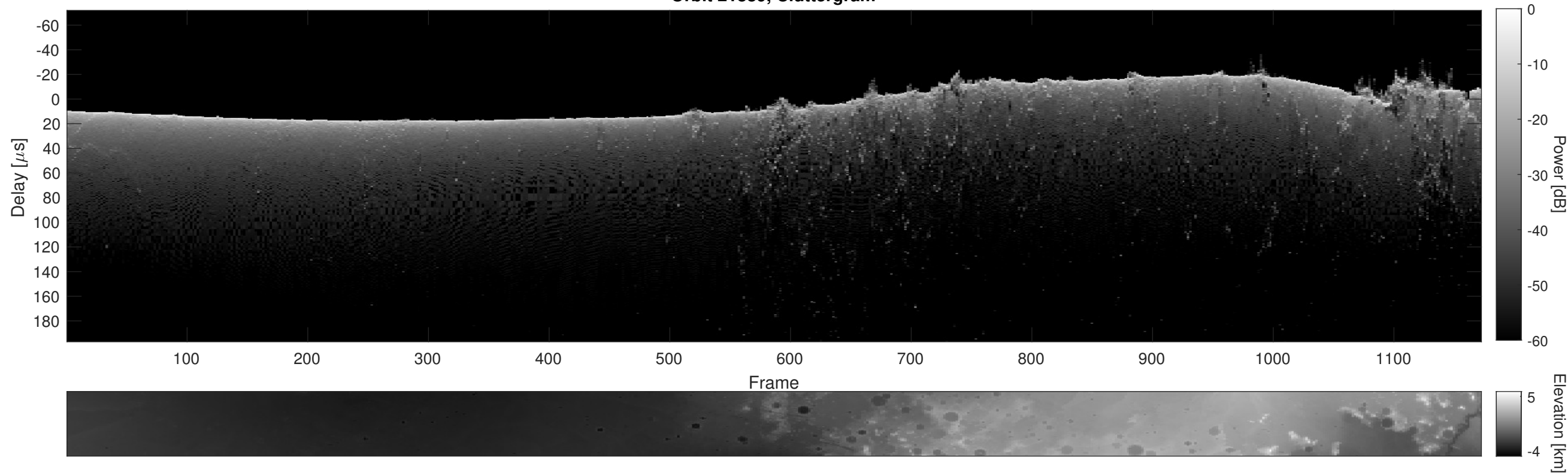
Orbit 21889, Cluttergram
