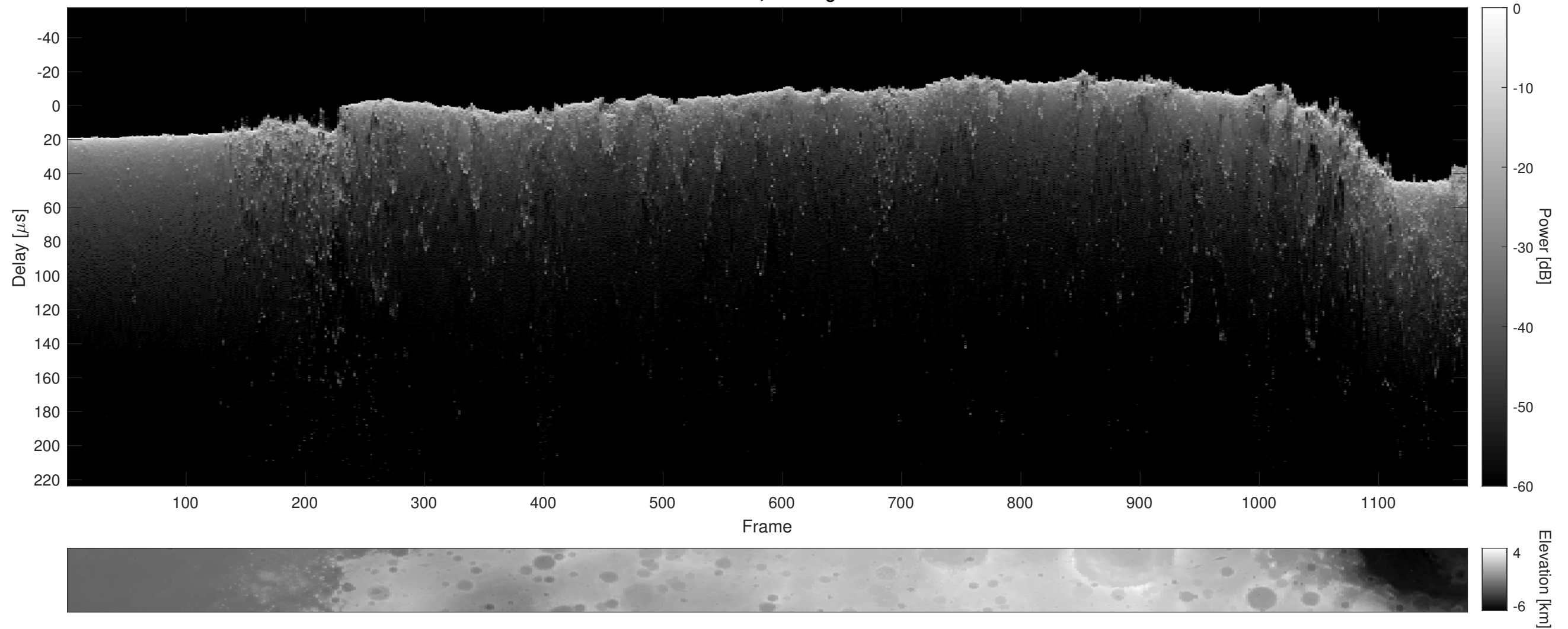
Orbit 21893, Cluttergram
