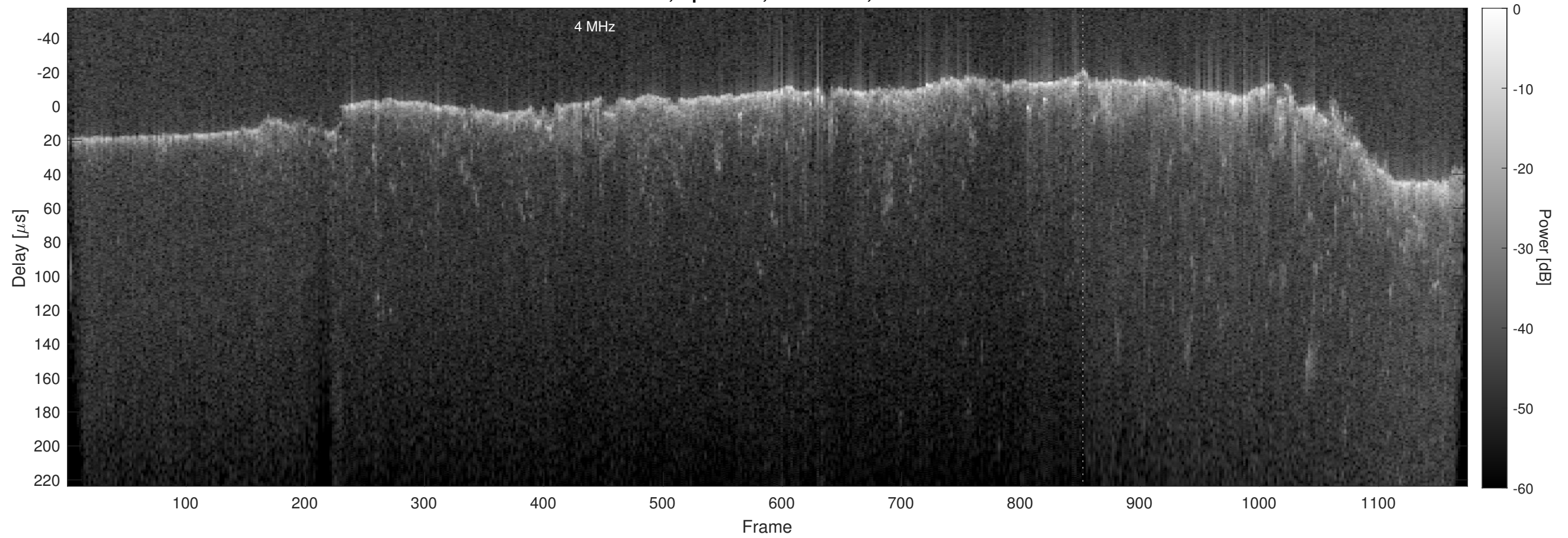
Orbit 21893, Optimized, No Window, Channel 2
