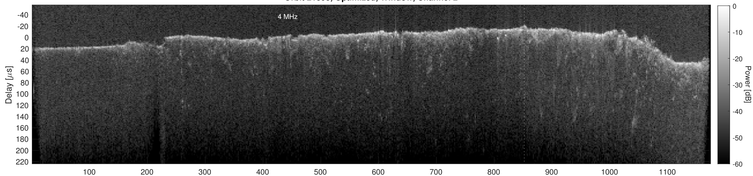
Orbit 21893, Cluttergram
