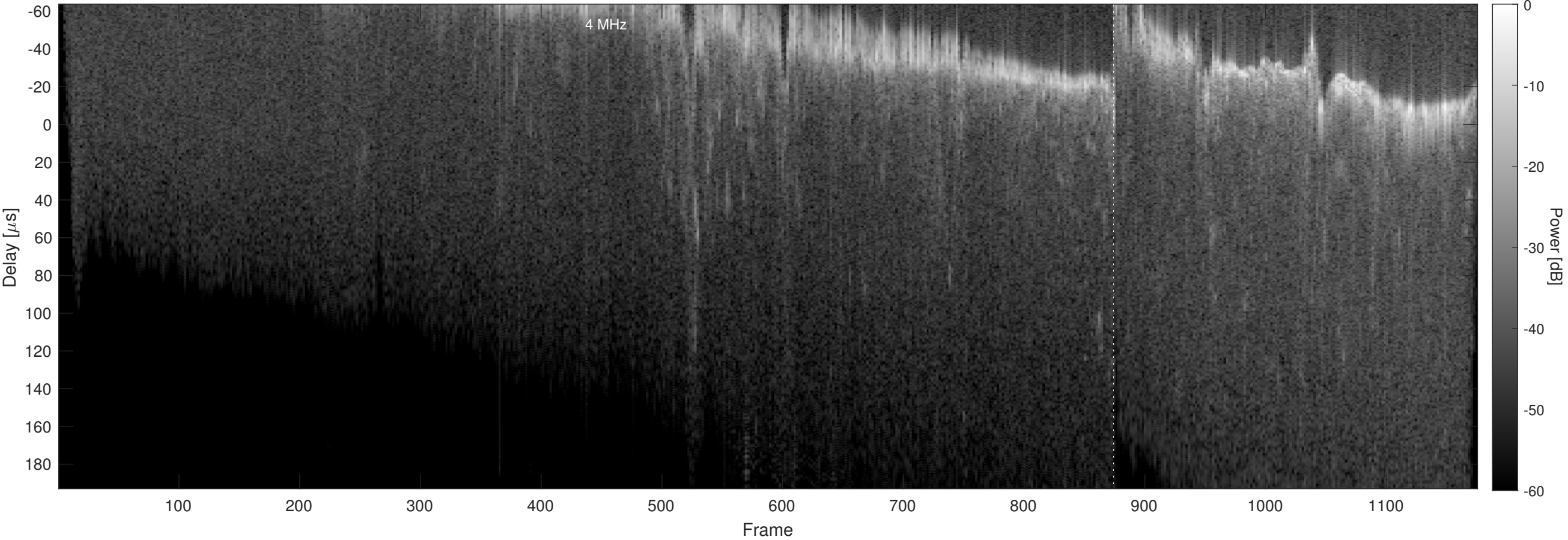
Orbit 21897, Chapman, No Window, Channel 2
