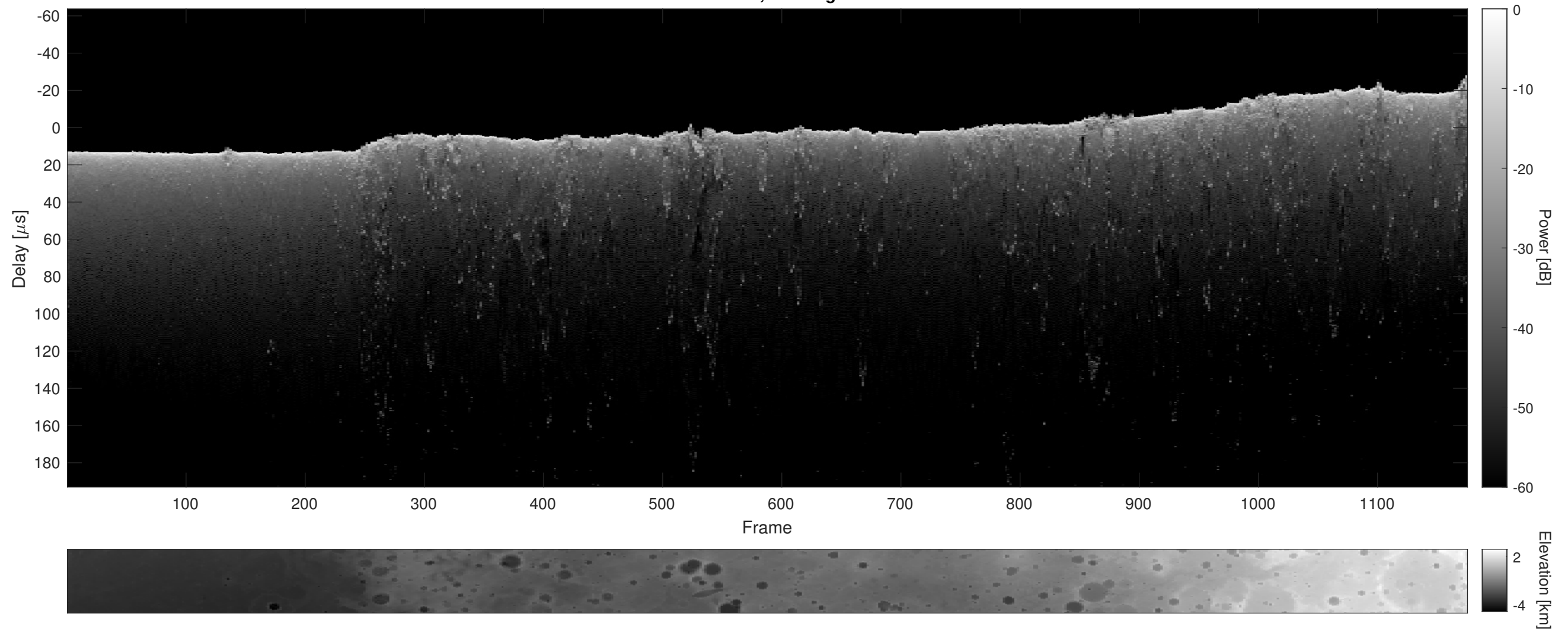
Orbit 21897, Cluttergram
