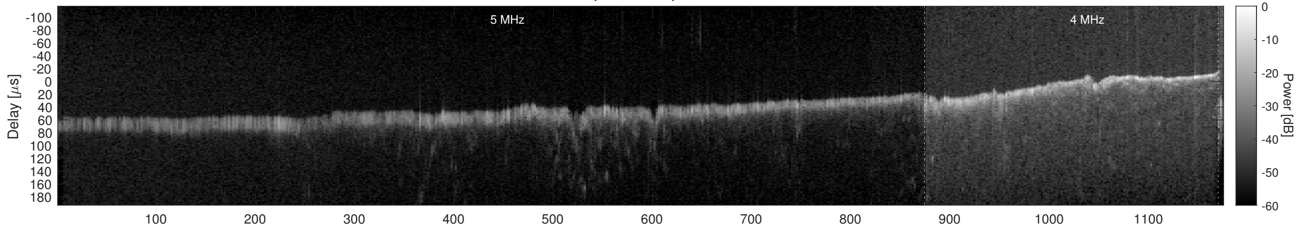
Orbit 21897, Window, Channel 1, Chapman
