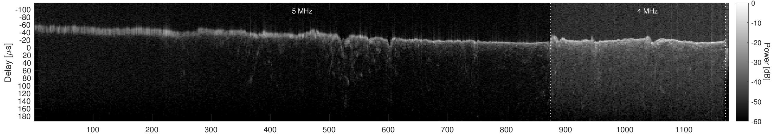
Orbit 21897, Window, Channel 1, Optimized
