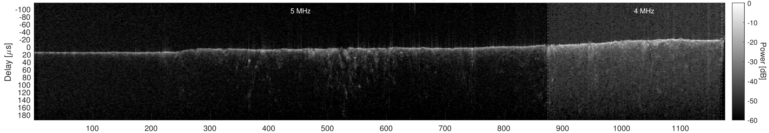
Orbit 21897, Cluttergram
