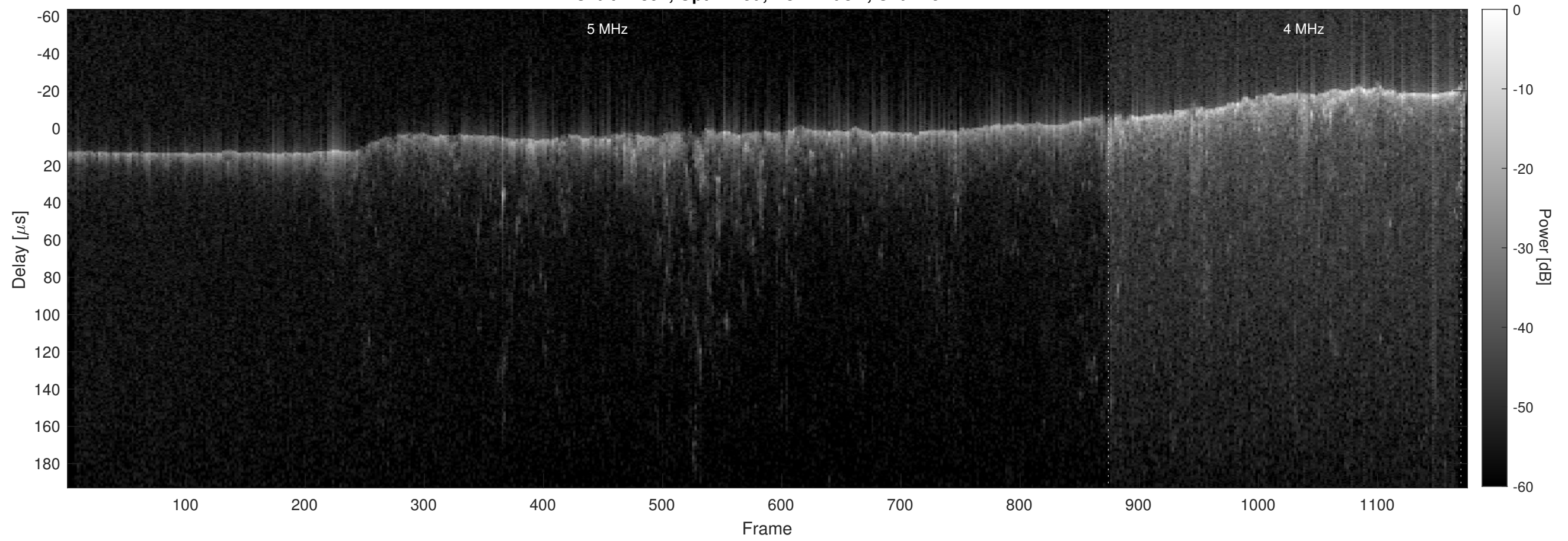
Orbit 21897, Optimized, No Window, Channel 2
