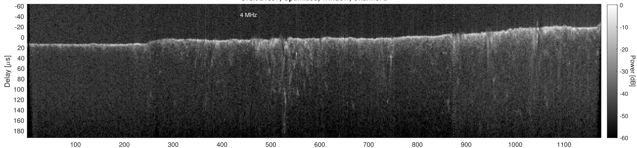
Orbit 21897, Cluttergram
