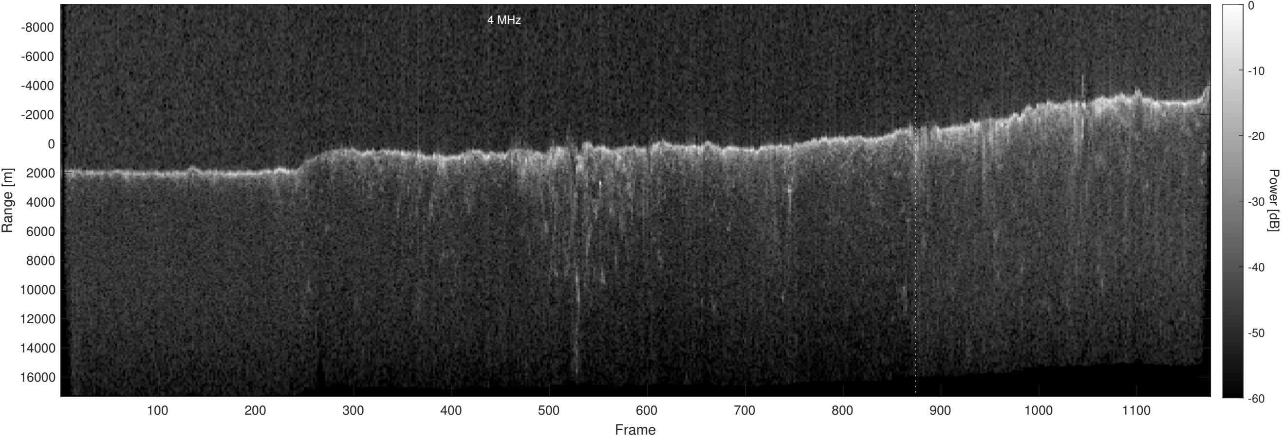
Orbit 21897, Optimized, Window, Depth-Corrected, Channel 2
