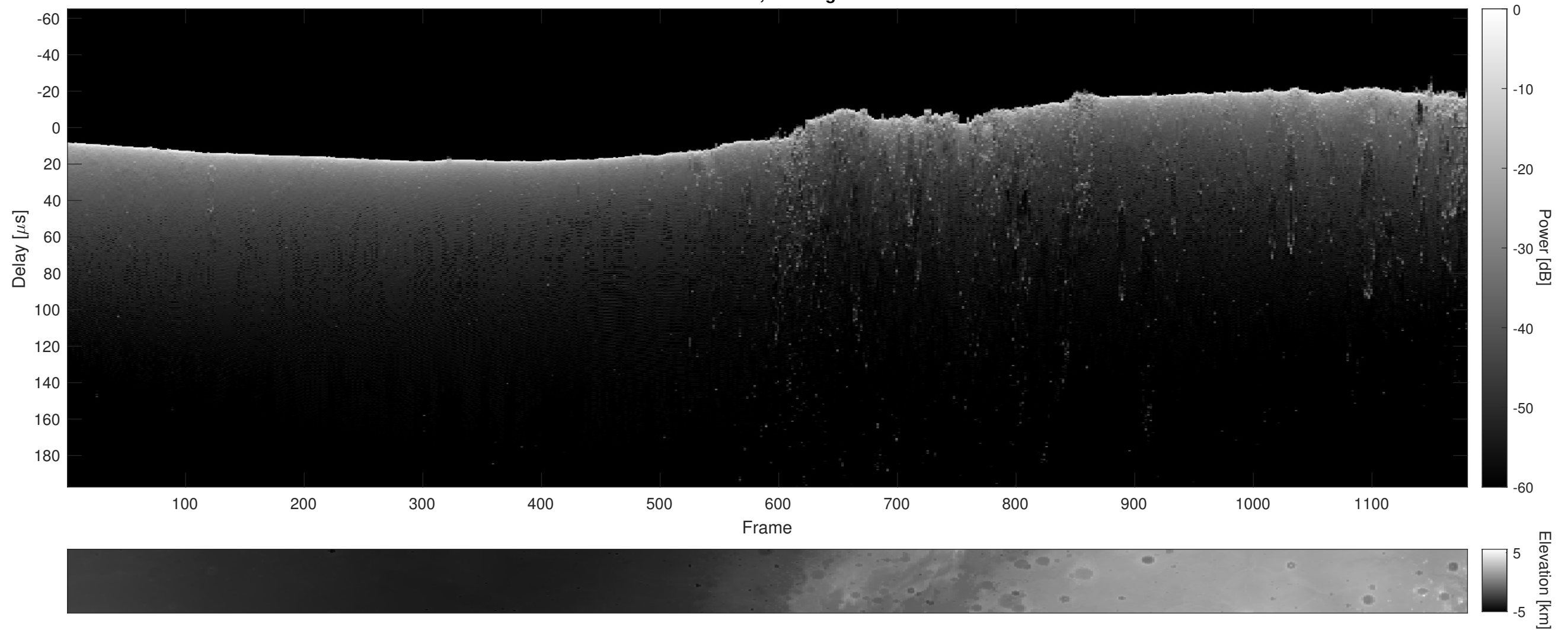
Orbit 21903, Cluttergram
