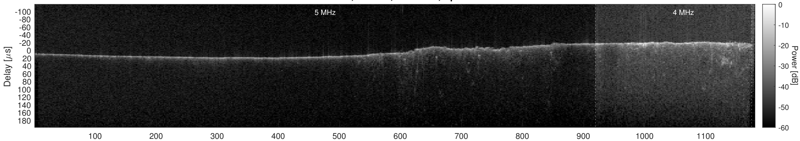
Orbit 21903, Cluttergram
