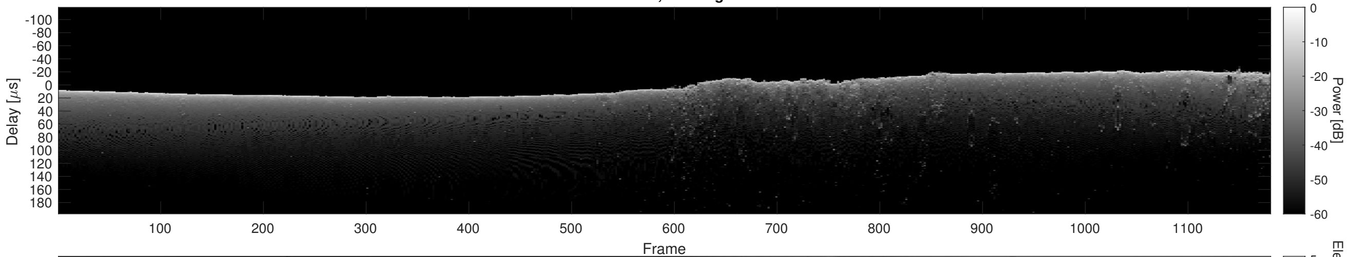
Orbit 21903, Cluttergram
