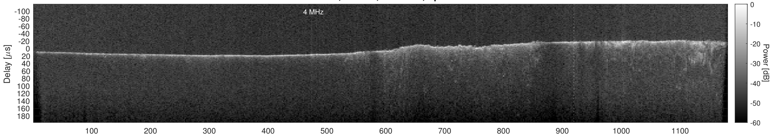
Orbit 21903, Cluttergram
