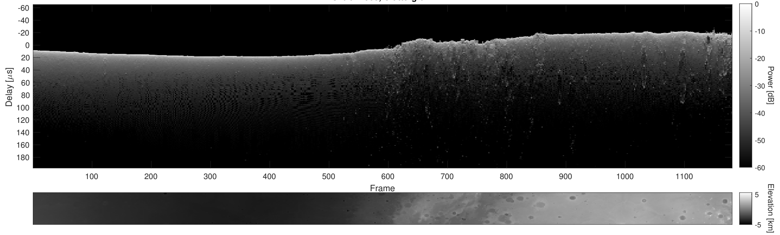
Orbit 21903, Cluttergram
