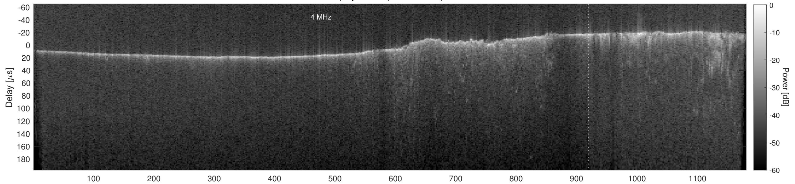
Orbit 21903, Cluttergram
