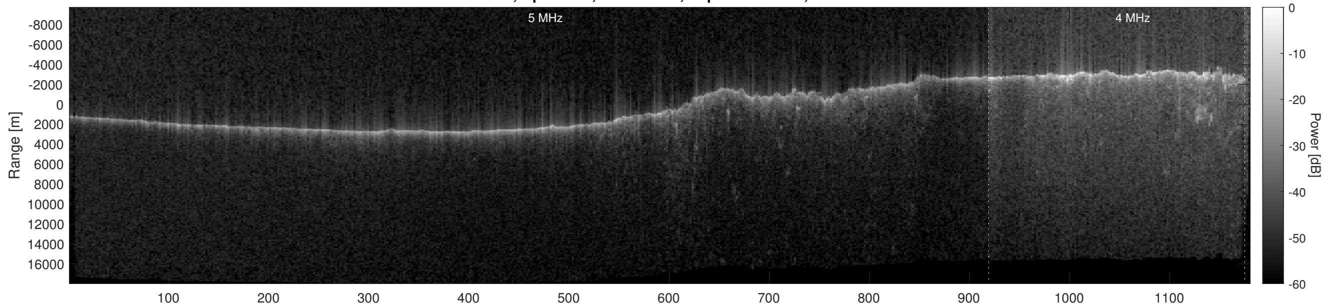
Orbit 21903, Optimized, No Window, Depth-Corrected, Channel 2
