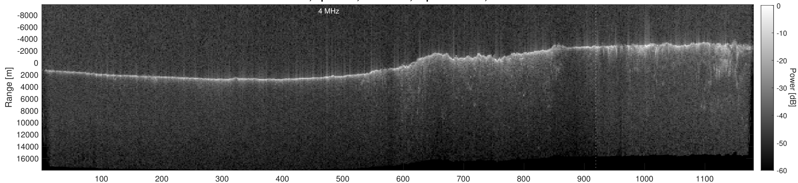
Orbit 21903, Depth-Corrected Cluttergram
