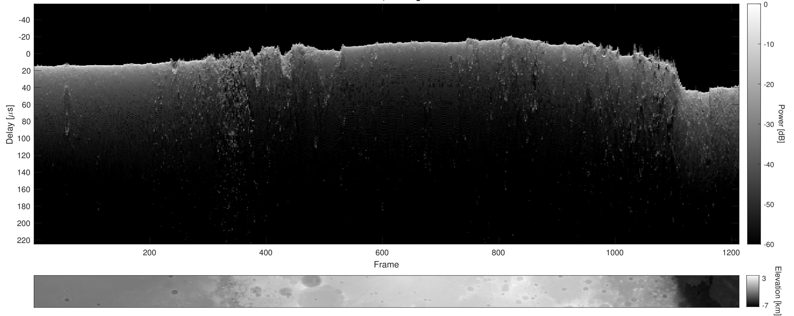
Orbit 21907, Cluttergram
