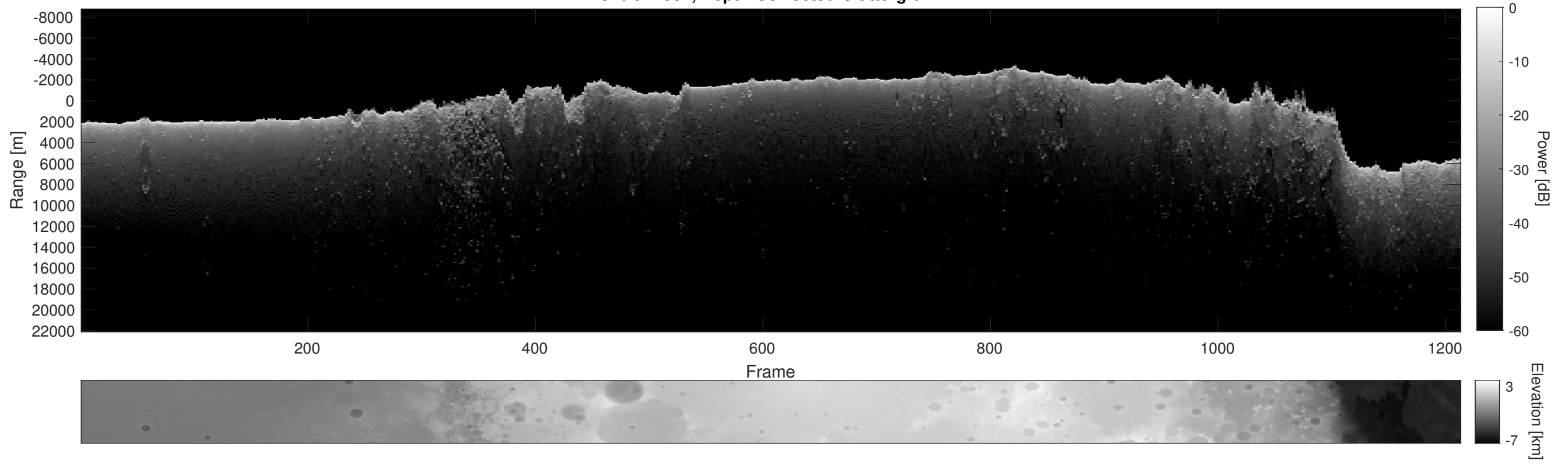
Orbit 21907, Depth-Corrected Cluttergram
